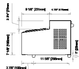
CPR-60-4 Side View
